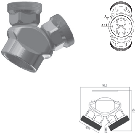
2-YV Y-Stück 50° Y-piece 50°
