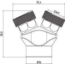
1-YV Y-Stück 50° Y-piece 50°
